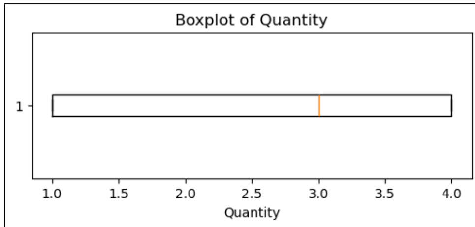
Boxplot: Quantity
