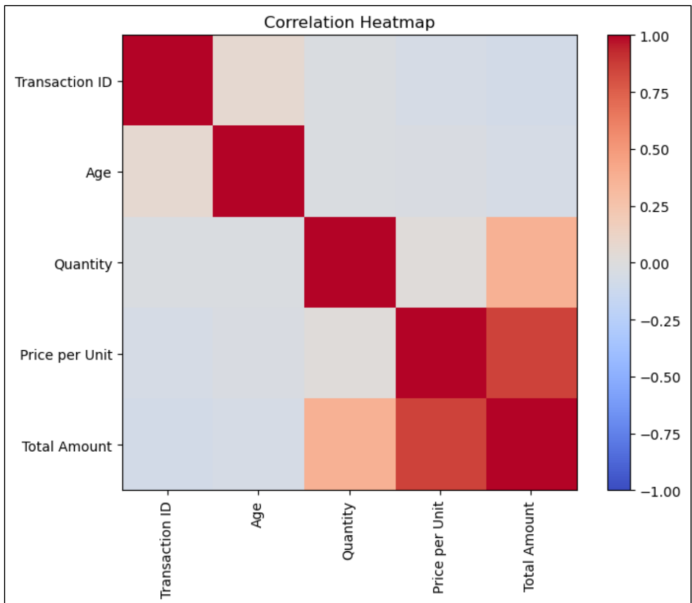
Correlation Heatmap
